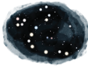
Drak
